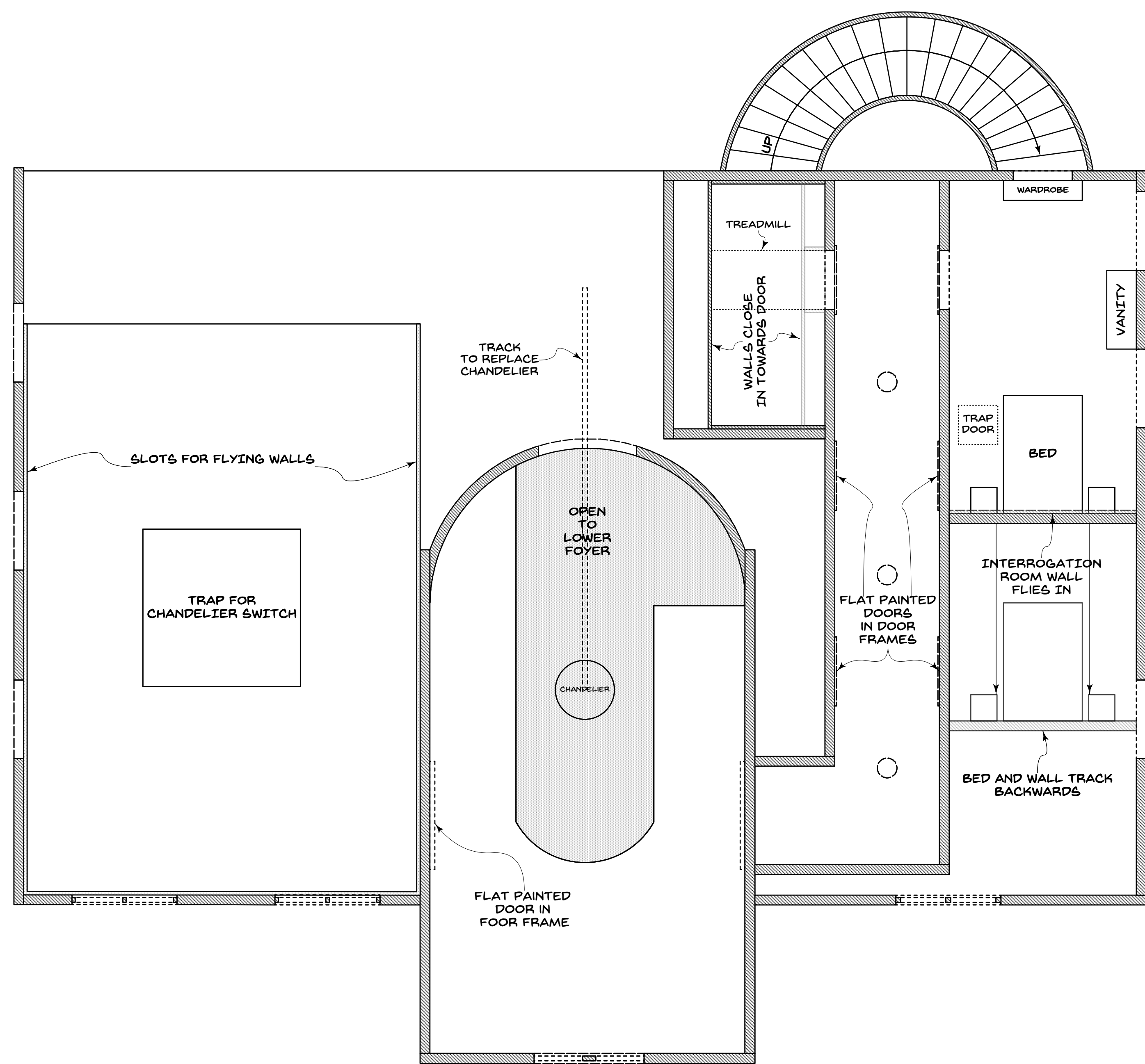
PLAN HOUSE 2ND FLOOR
