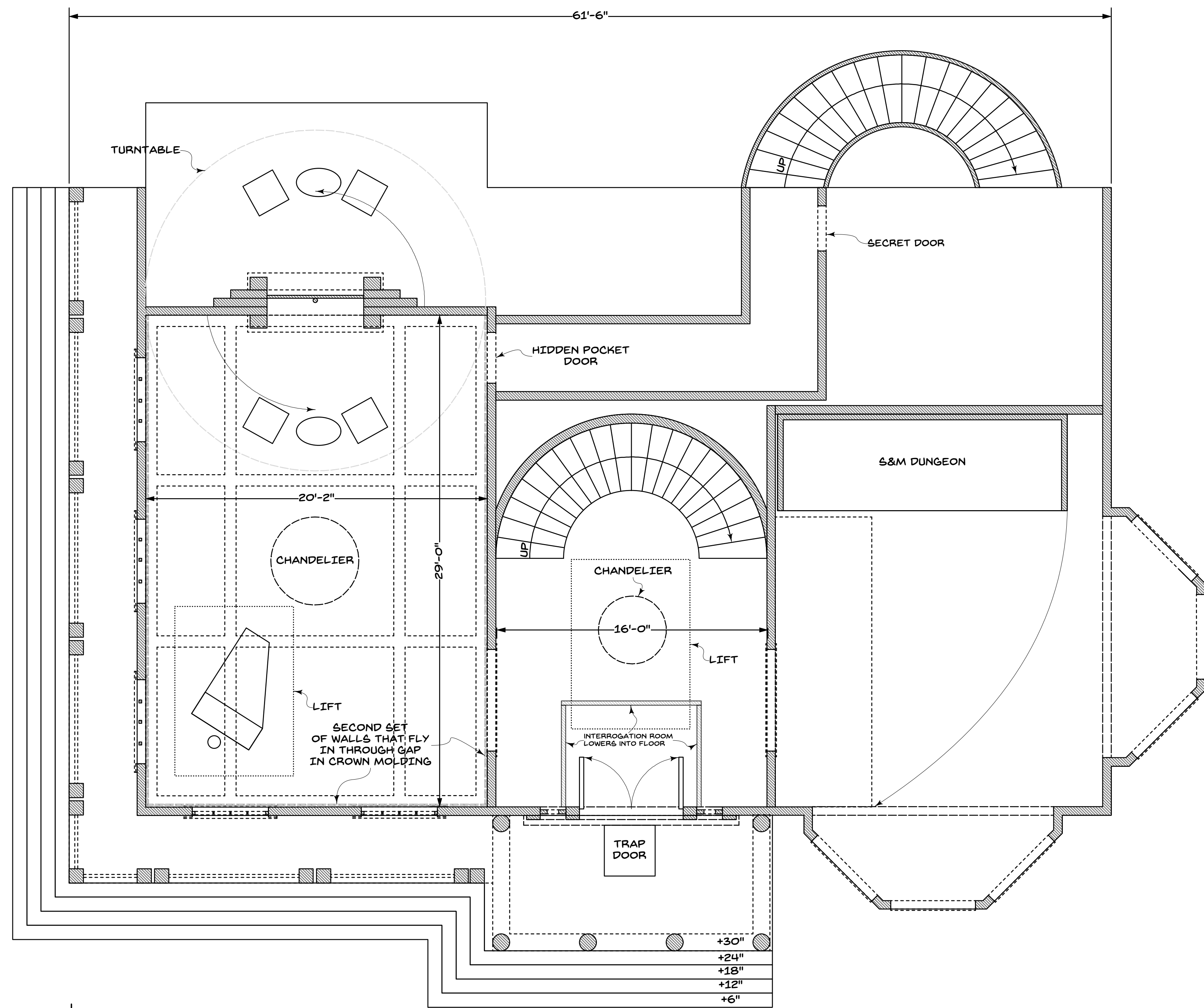
PLAN HOUSE 1ST FLOOR
